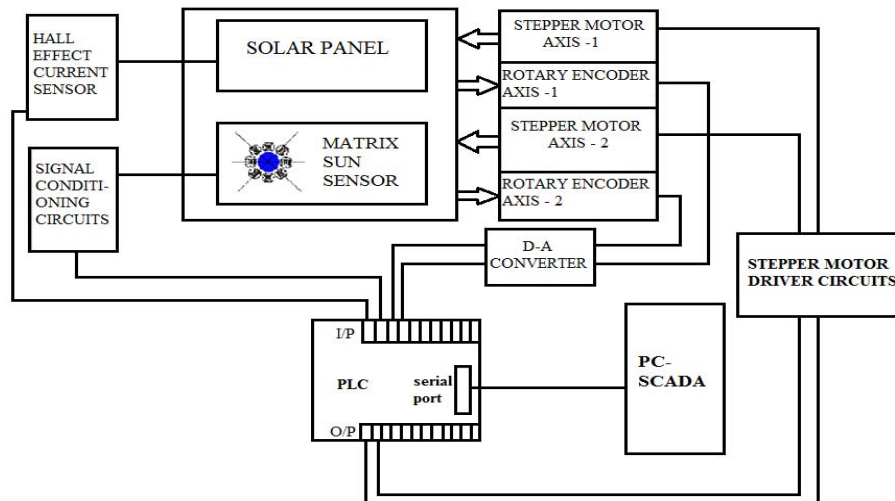
Figure 2. Block Diagram of the Proposed Technique
