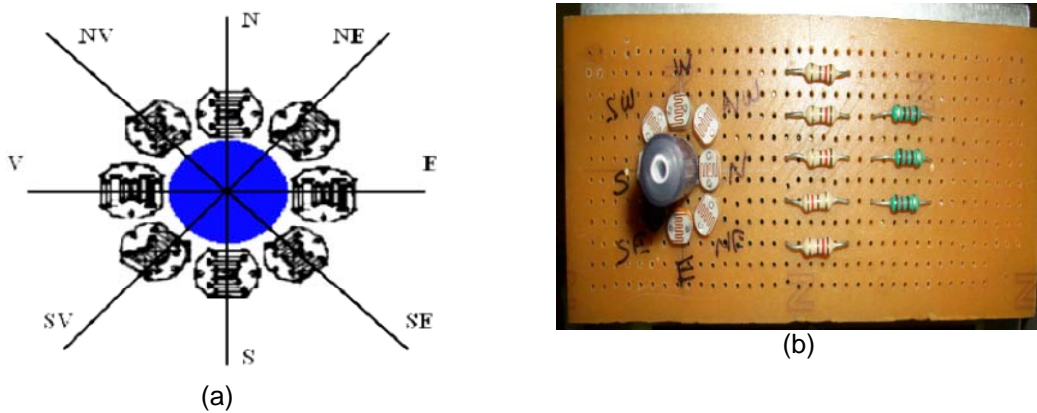
Figure 3. (a) Pictorial representation of MSS, (b) Actual photograph of MSS
