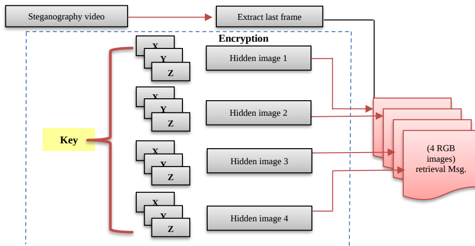
Figure 3. General structure of decoding and masking
