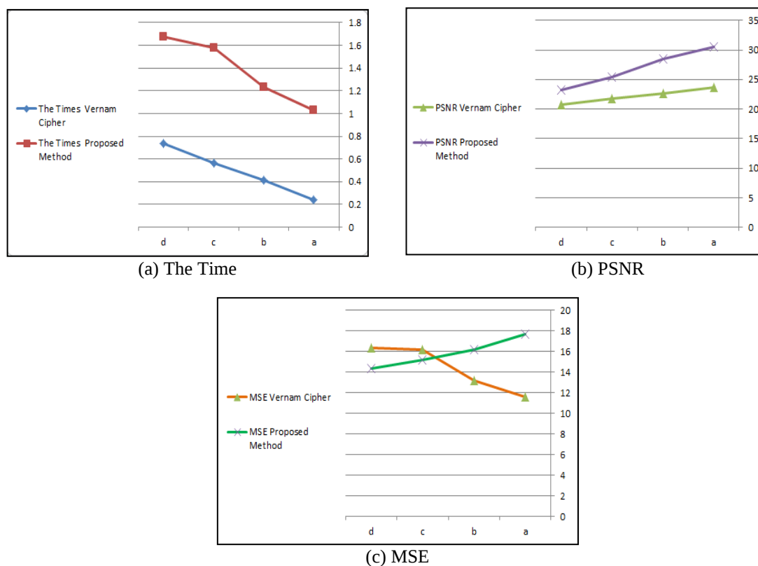
Figure 7. The different between Vernam cipher and proposed method (a) the times, (b) PSNR, and (c) MSE
