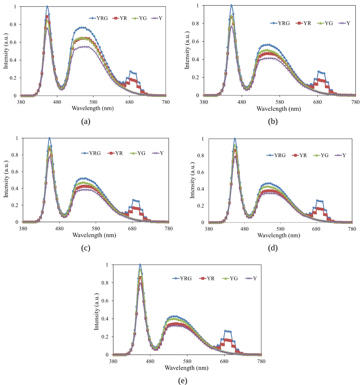
Figure 3. The emitting spectrum for each remote phosphor structure at different ACCTs (a) 5,600 K, (b) 6,600 K, (c) 7,700 K, (d) 7,700 K, and (e) 8,500 K
