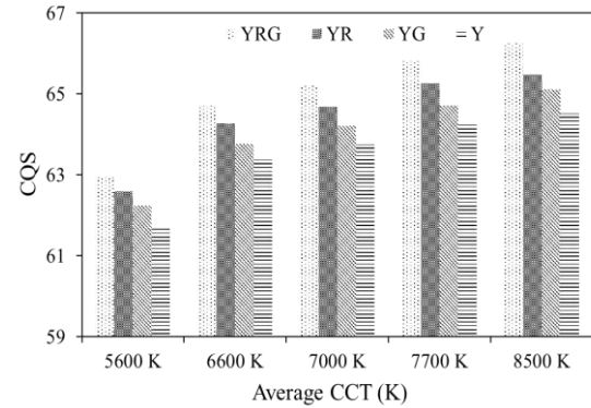
Figure 5. CQS of phosphor settings under various ACCTs
