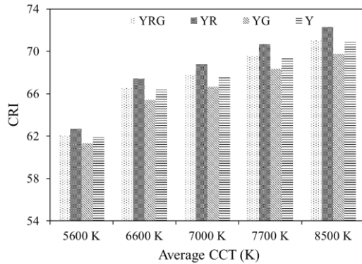
Figure 4. CRI values for phosphor settings under various ACCTs
