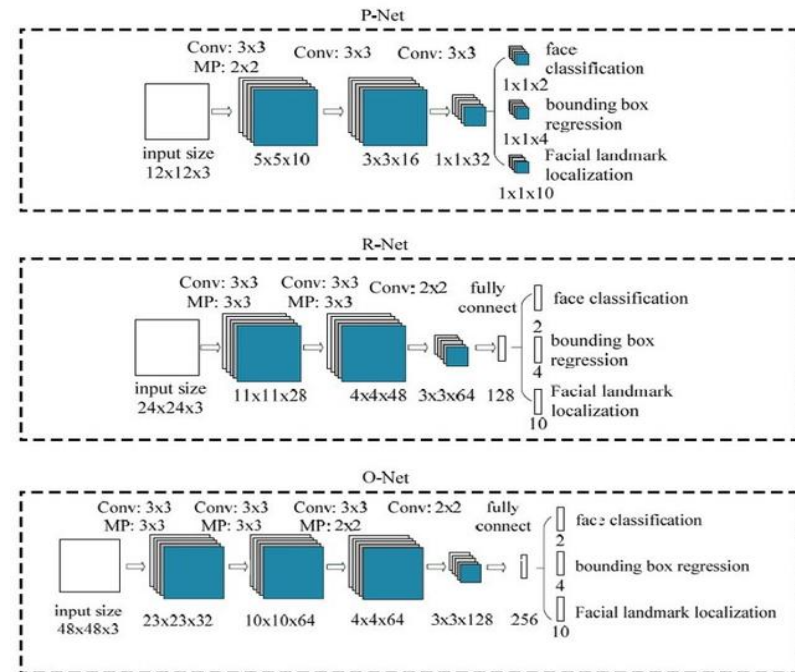
Figure 4. The three stages of MTCNN [17]
