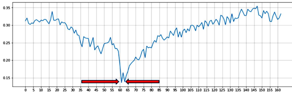
Figure 2. The initial blink is recognized using a single blink detection technique between frames 60 and 65
