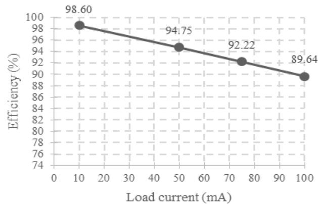
Figure 14. Measured efficiency
