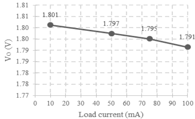
Figure 13. Measured load regulation
